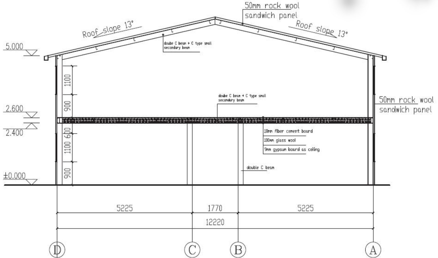
Drawing for senior expats building
