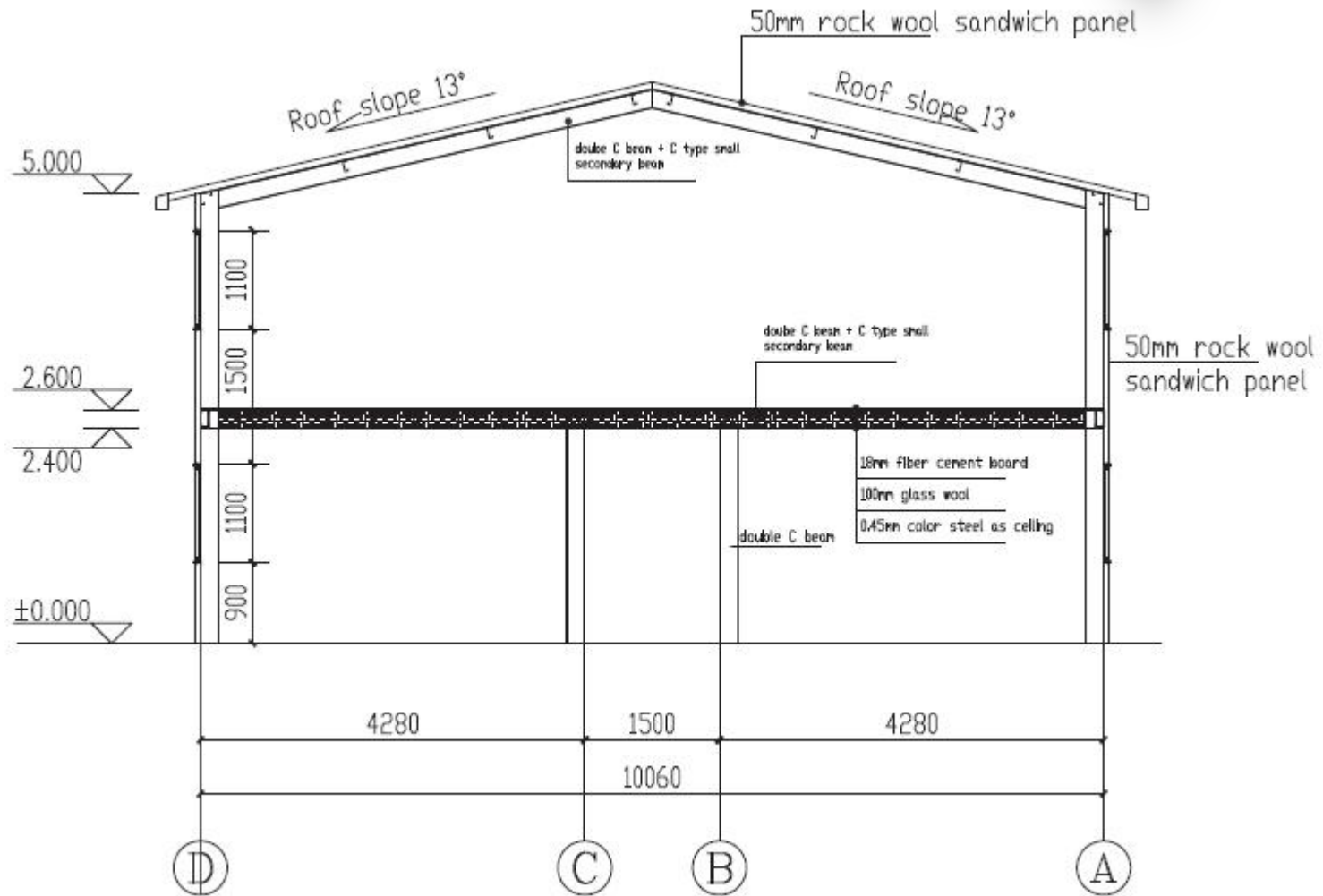
Drawing for expats building
