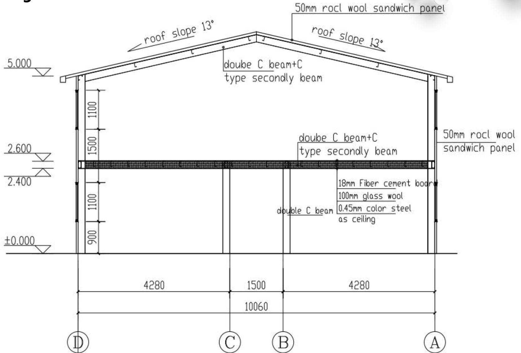
Drawing for worker block
