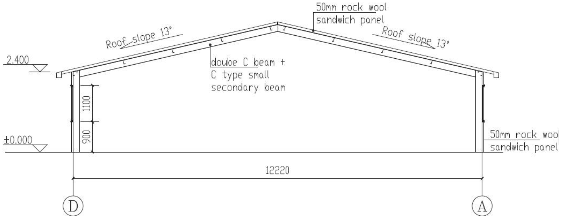
Drawing for canteen
