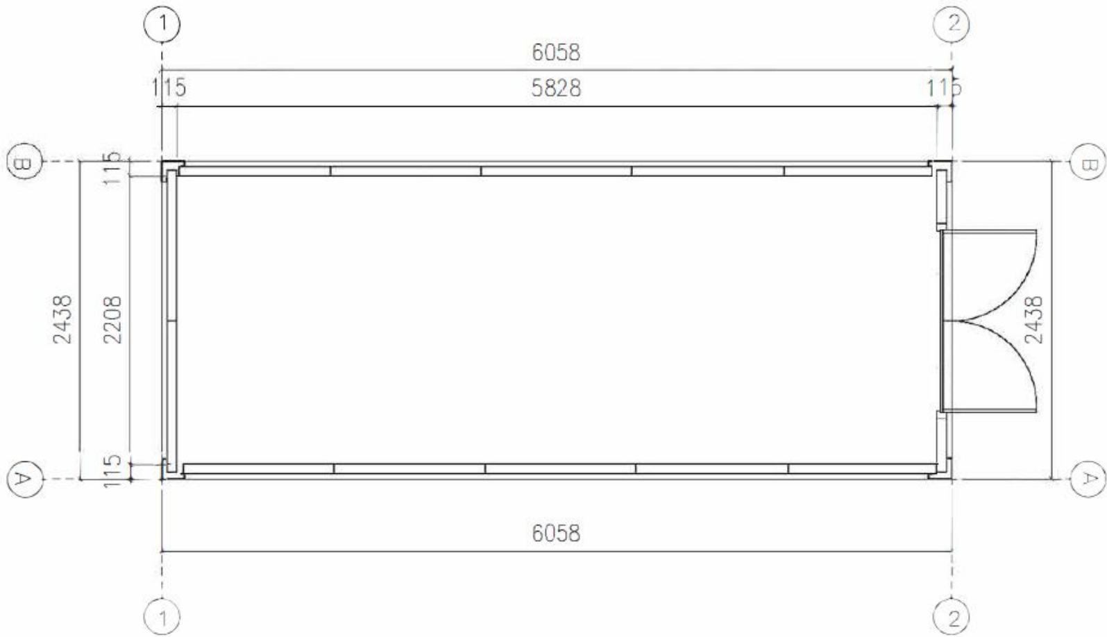
Waste container
