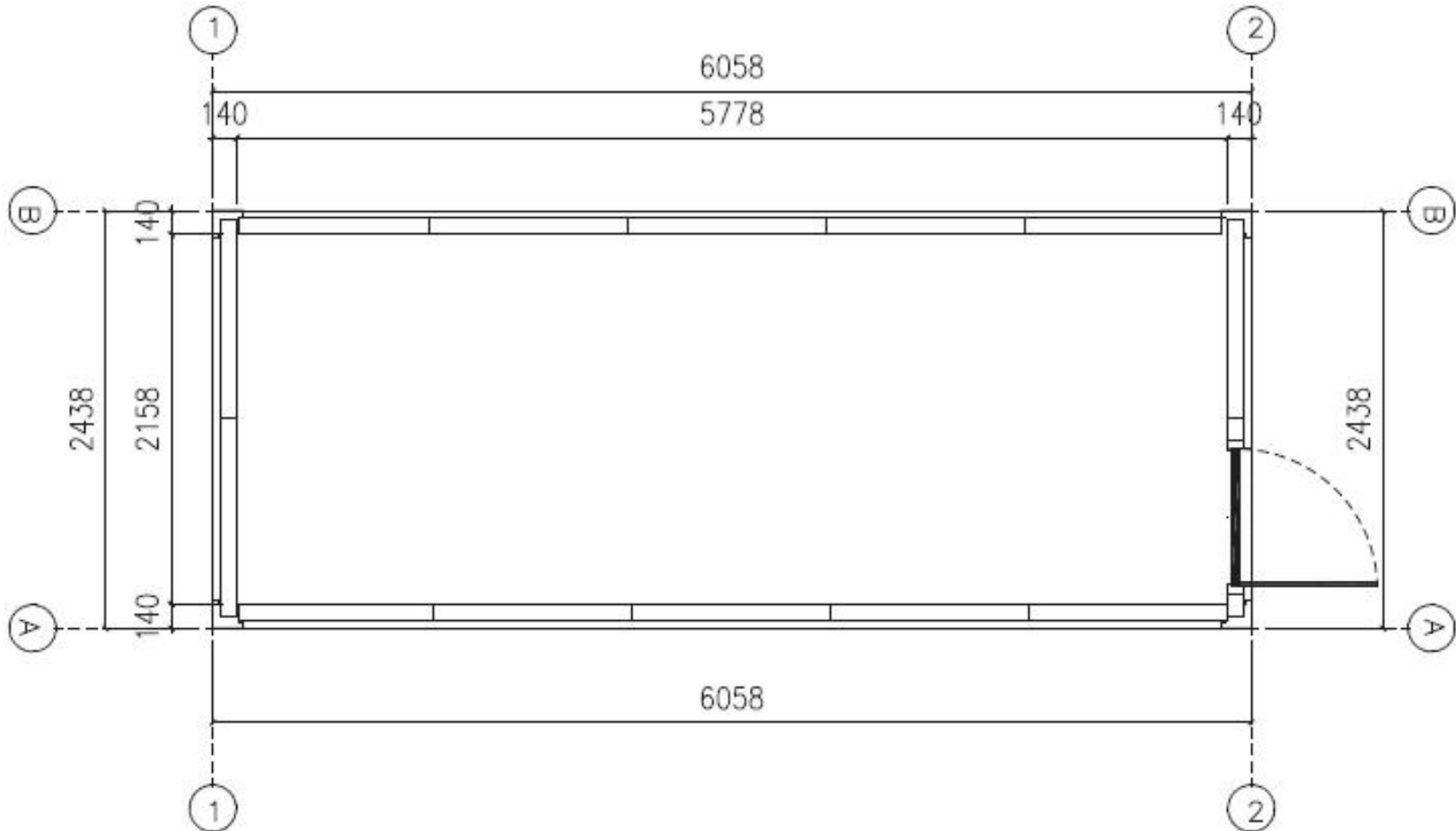
Chiller container
