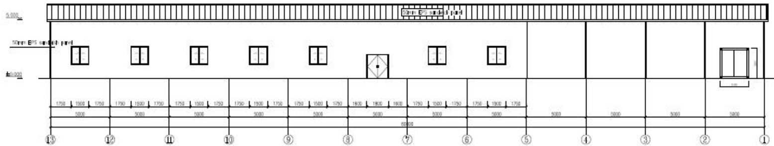
D axis elevation 1:100
