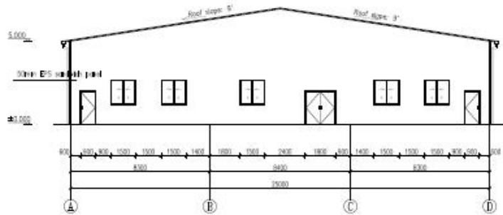
13 axis elevation 1:100
