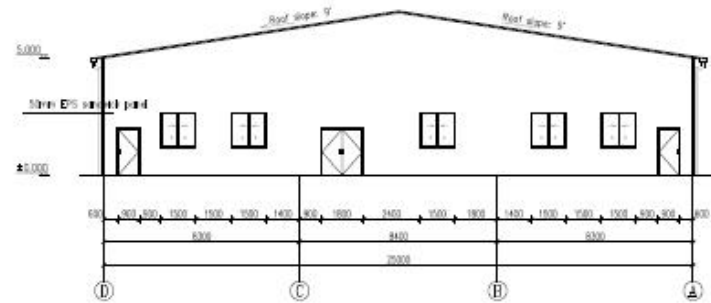
5 axis elevation 1:100
