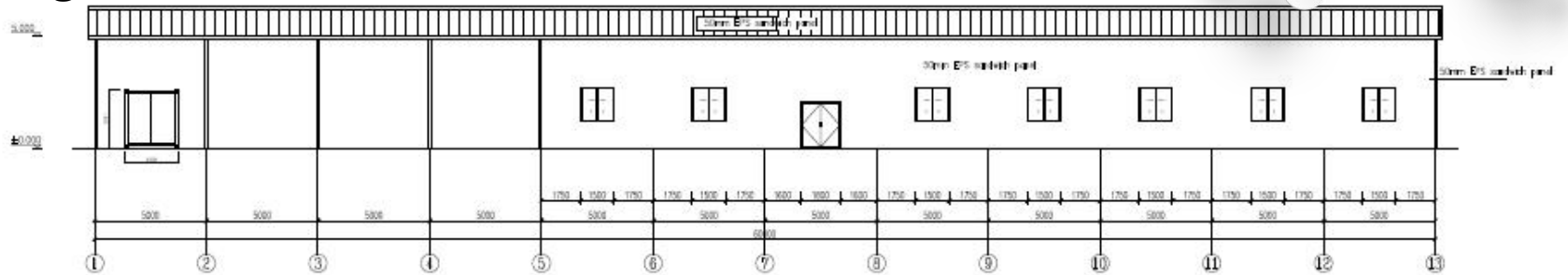
A axis elevation 1:100
