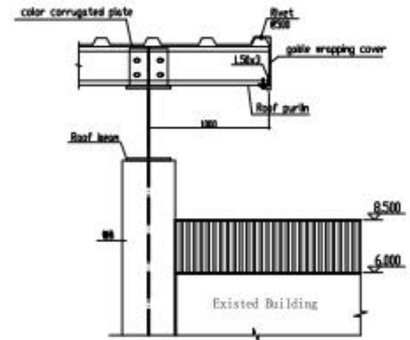
Connection details of roof purlin, gable wall angle steel and trimming
